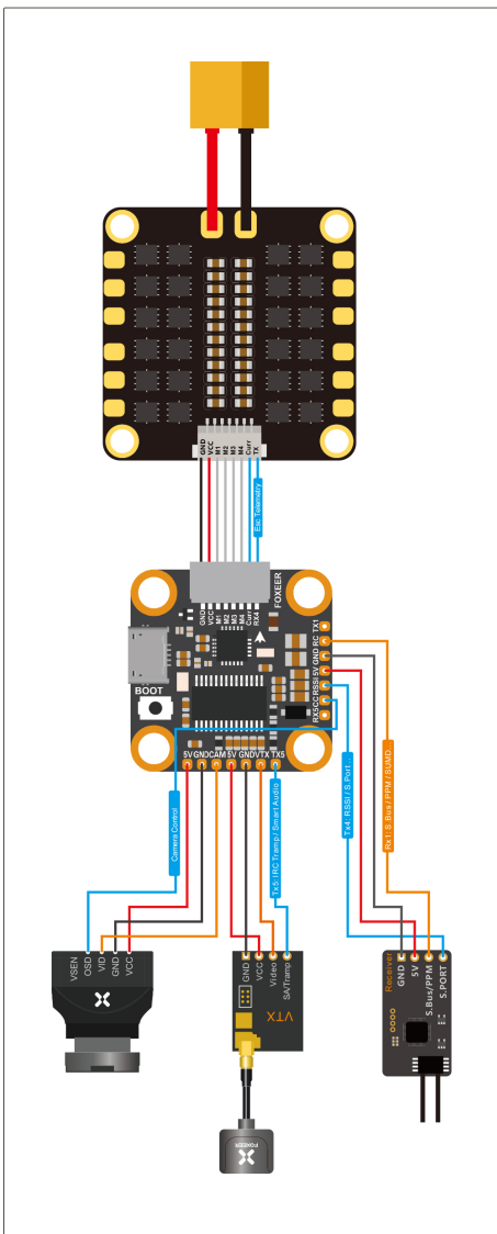
Wiring schematic diagram
